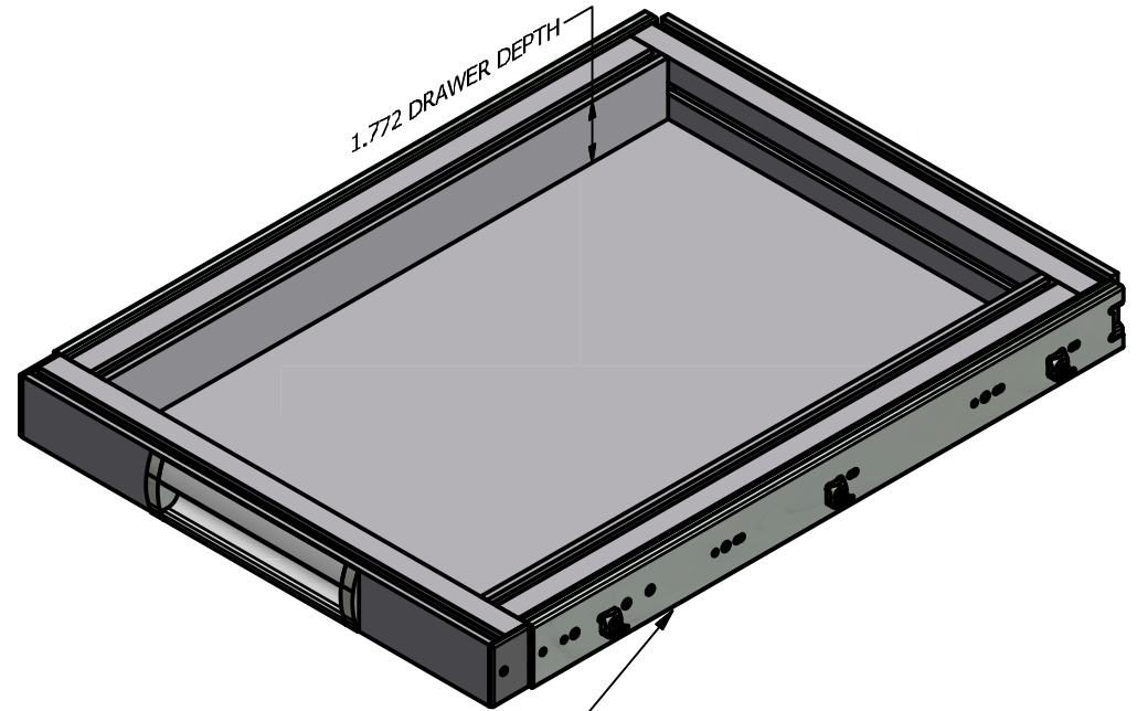
20" TRAVEL DRAWER SLIDE 95 LB/PAIR LOAD RATING
